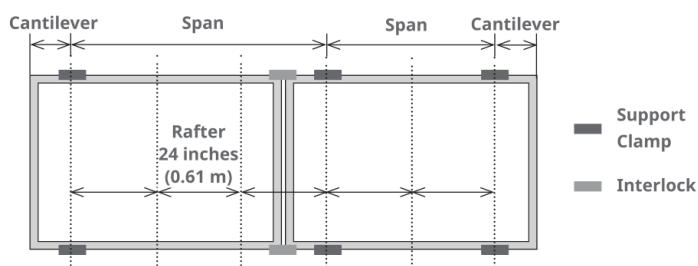
Landscape installation, clamping on long side frame
